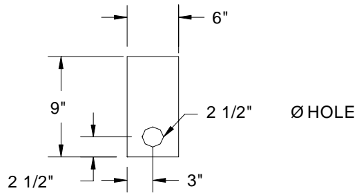
WEIR SPLICE PLATE DETAIL
