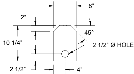
WEIR SPLICE PLATE DETAIL
