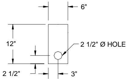
WEIR SPLICE PLATE DETAIL
