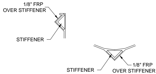
EMBEDDED STIFFENER DETAILS
