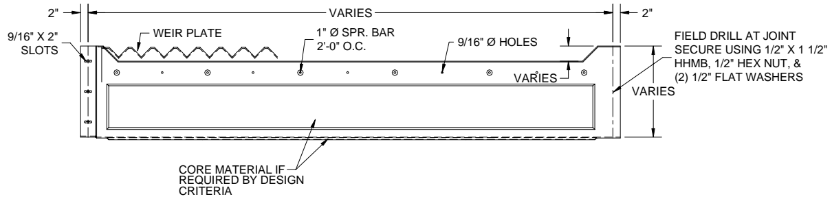
ELEV. VIEW BACK TROUGH – ASSEMBLED
