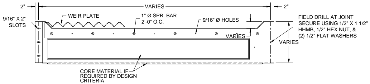
ELEV. VIEW FRONT TROUGH – ASSEMBLED
